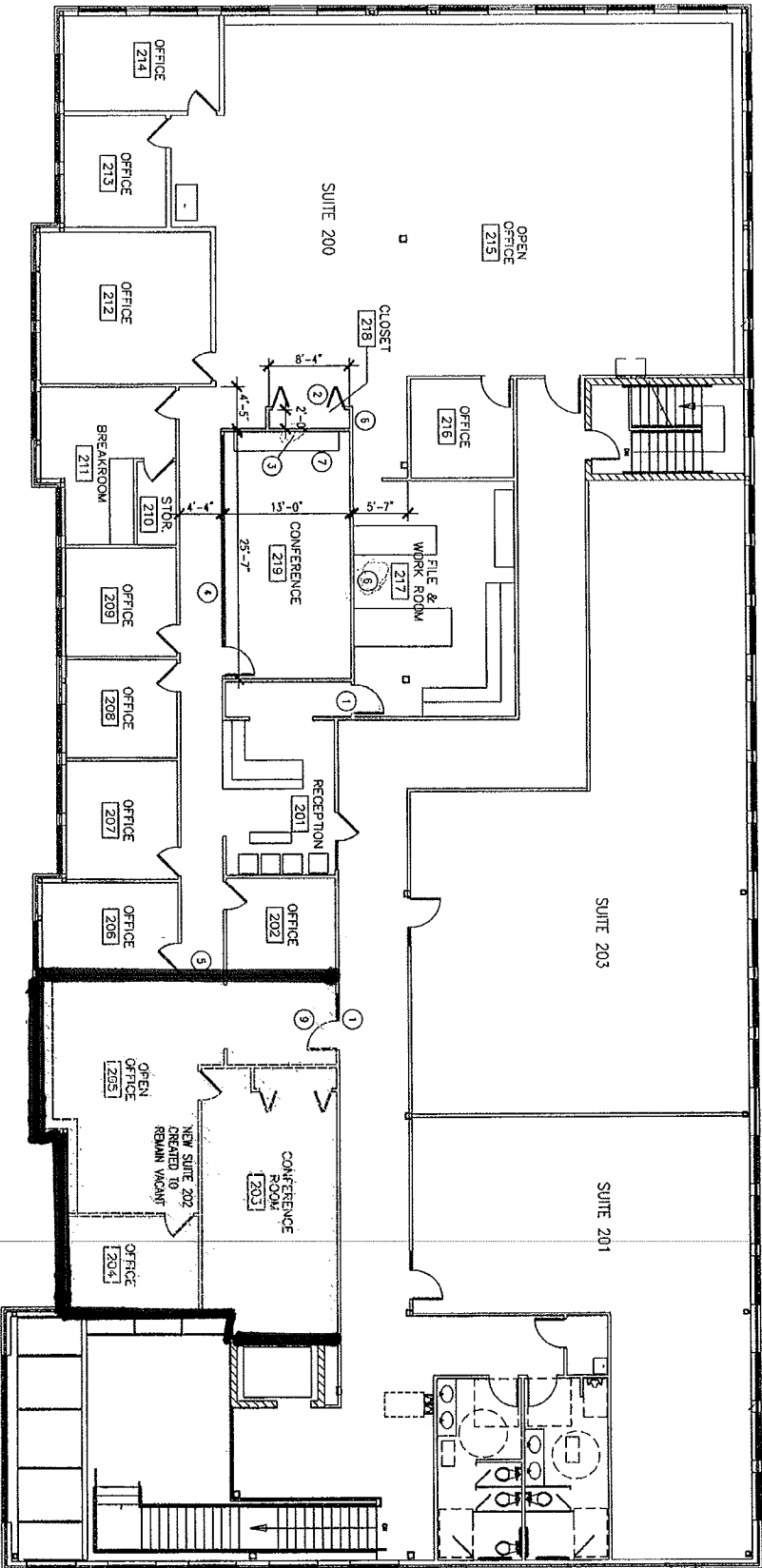
2 7/8" = 1'-0" FLOOR PLAN - SECOND FLOOR
